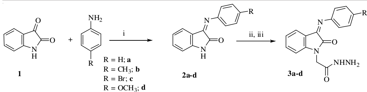
Scheme-II: 2-(2-Oxo-3-(4-substituted phenylimino)-indolin-1-yl)acetohydrazide derivatives 3a-d : Reaction conditions: (i) MW/80 °C/400 watts/2 min. (ii) ethylchloroacetate/ \text{K}_2\text{CO}_3 /acetone/MWI/60 °C/600 watts/10 min. (iii) \text{NH}_2\text{NH}_2 (99 %)/MeOH/MWI/ 60 °C/400 watts/2 min
