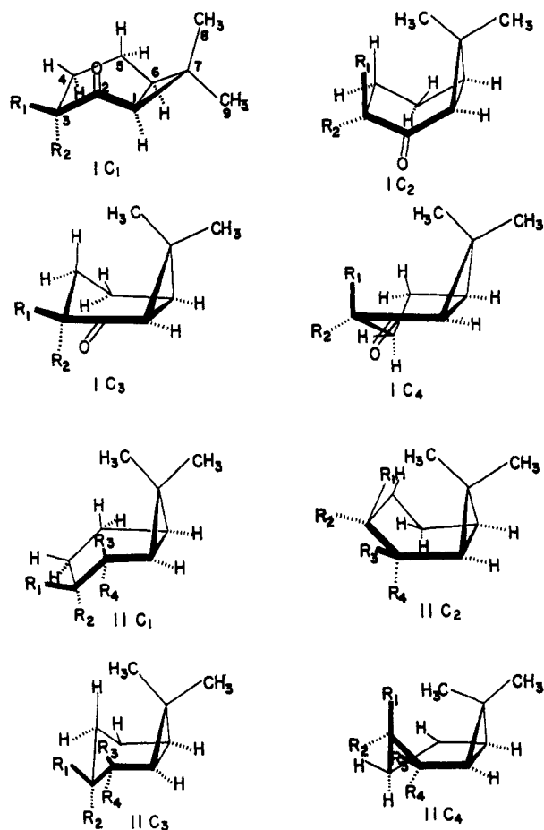
Figure 5. Possible conformations for the 2-caranones and 2-caranols.
