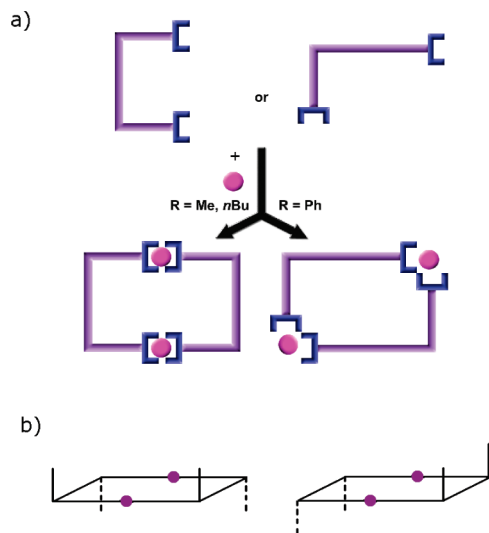
Scheme 2. Graphical Illustration of (a) the Differences in the Tin–Atom Configurations and Ligand Conformations and (b) the Conformational Ring Isomerism Found in Compounds 1 , 4 , 5 , and 6
