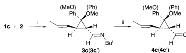
Scheme 2 Reagents and conditions: i, THF, 60 °C, 14 h; ii, SiO 2 , hexane–EtOAc (4 : 1)
