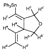
7 (NMR assignment)
