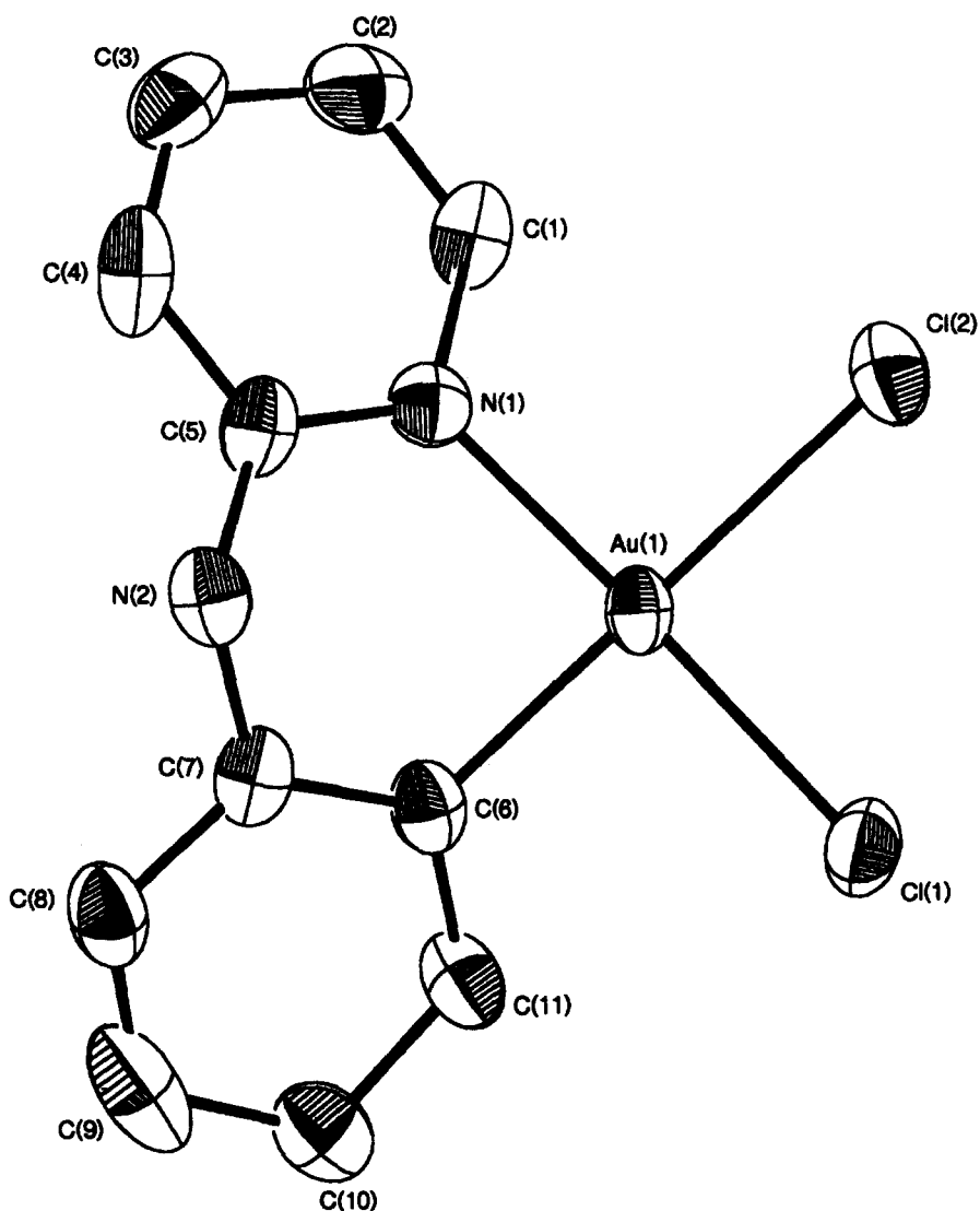
Fig. 1. ORTEP drawing of [\text{AuCl}_2(\text{anp})] and atom labelling scheme.
