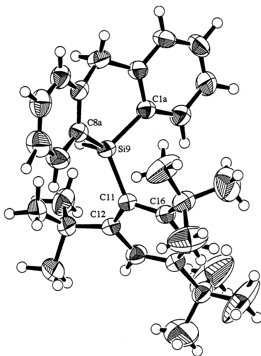
Fig. 1. Molecular structure of 1g . Important bond lengths (Å) and angles ( ^\circ ): Si(9)–C(1a) = 1.869(3), Si(9)–C(8a) = 1.871(3), Si(9)–C(11) = 1.896(3); C(1a)–Si(9)–C(8a) = 104.2(1) , C(1a)–Si(9)–C(11) = 112.0(1) , C(8a)–Si(9)–C(11) = 122.8(1) , Si(9)–C(11)–C(12) = 117.4(2) , Si(9)–C(11)–C(16) = 122.7(2) , C(12)–C(11)–C(16) = 116.8(3) .
