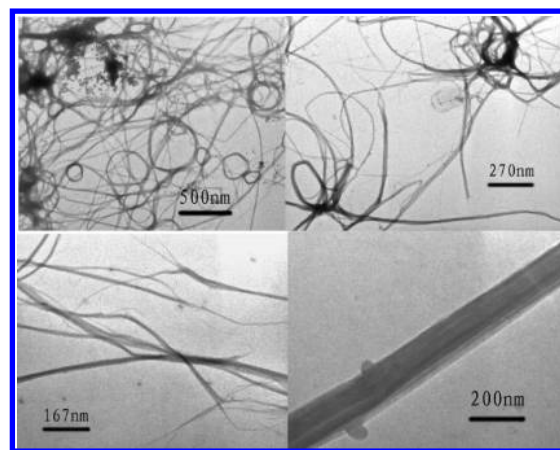
Figure 2. TEM micrographs of TP1 nanofiber suspension drop-casted and dried on a 200-mesh copper grid covered with a carbon film.
