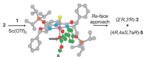
Figure 2. The assumed reactive intermediate 6 in the DA and HDA reactions between 2 and Cp catalyzed by the Sc(OTf) 3 complex of pybox 1 , which gives (2 R ,3 R )- 3 and (4 R ,4 a ,5,7 aR )- 5 . pybox = pyridinebis(oxazoline).
