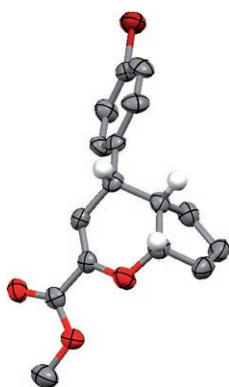
Figure 1. X-ray structure of 5c , thus confirming the absolute 4 R ,4 a ,5,7 aR configuration.
