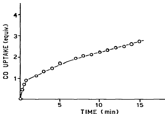
Fig. 1. Carbonylation of the complex \text{Ni}(\text{CN})(\text{C}_6\text{H}_5)(\text{PET}_3)_2 ( 10^{-2} M ) in decalin at 25^\circ\text{C} in the presence of 10^{-2} M \text{ PET}_3 .
