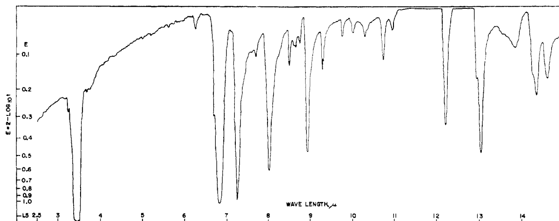
Fig. 5.—Infrared spectrum of N,N'-diphenyl- p -quinonediimine-N,N'-dioxide.
