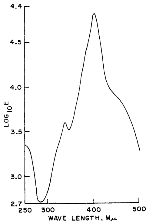
Fig. 6.—Spectrum of N,N'-di( sec -butyl)- p -quinonediimine-N,N'-dioxide.
