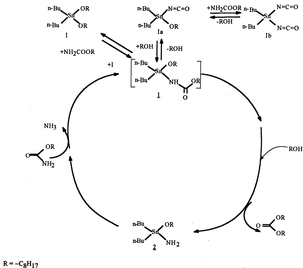
Scheme 4. Proposed reaction mechanism for the formation of a dialkyl carbonate from an alkyl carbamate.
