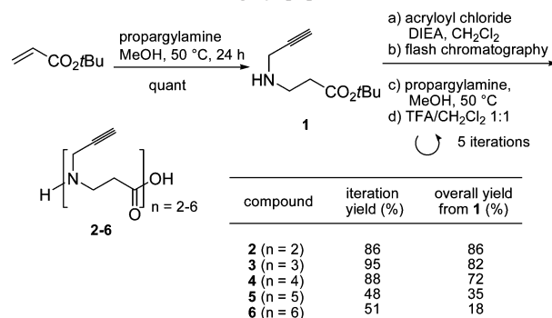
Scheme 1. Iterative Solution-Phase Synthesis of Oligo- \beta -peptoids
