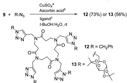
Scheme 2. Functionalized Cyclic \beta -Peptoids
