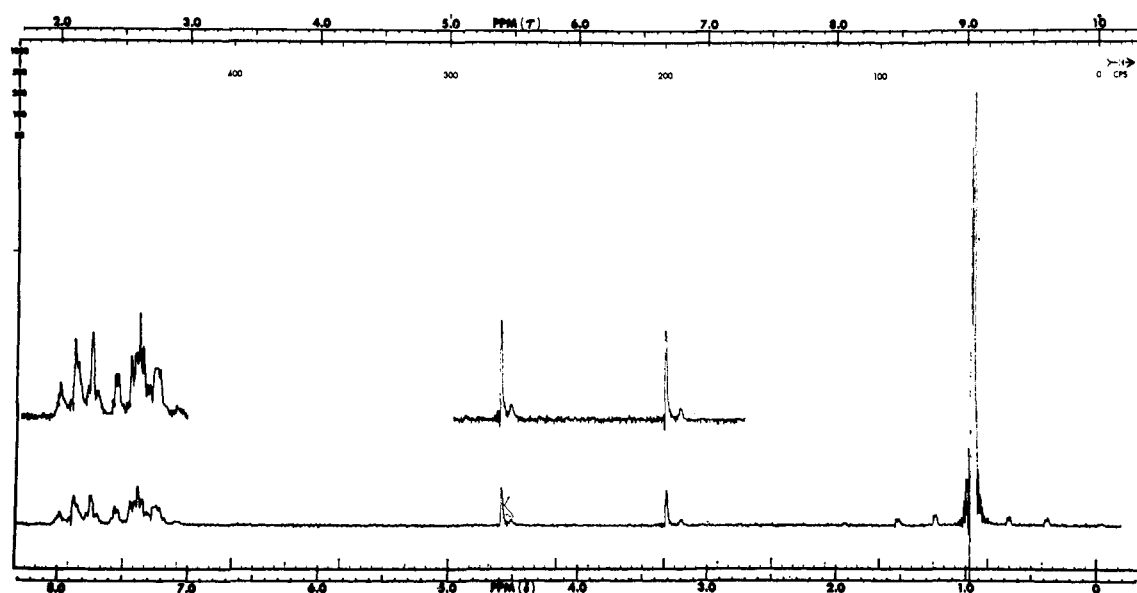
Figure 2. Complete proton magnetic resonance spectrum at 60 Mcps and 35°C of N-trimethylsilylaniline- N^{15} .
