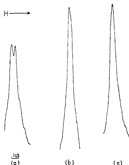
Figure 5. The methyl proton regions of the proton magnetic resonance spectrum of N-trimethylsilylaniline- N^{15} at 40 Mcps (a) without irradiation, (b) with irradiation at 4,053,533.2 \pm 0.5 cps, and (c) with irradiation at 4,053,456.4 \pm 0.5 cps.
