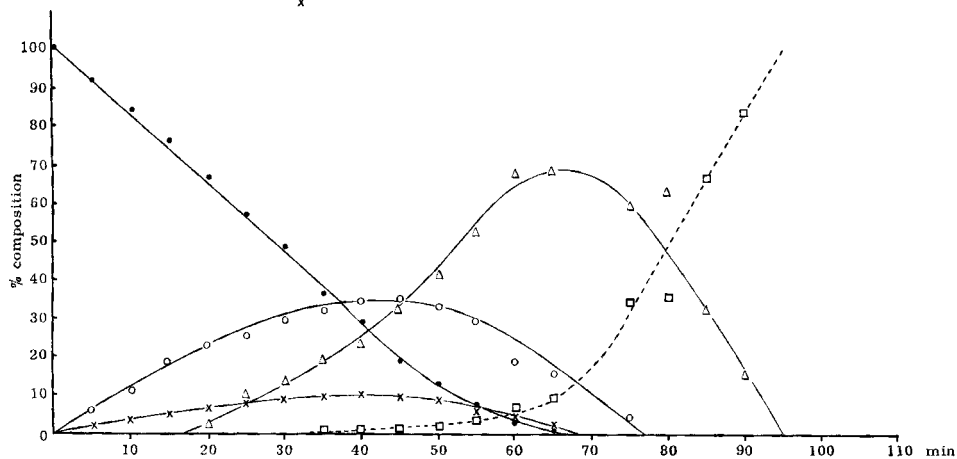
Ozonization of (-)\beta -Elemene
