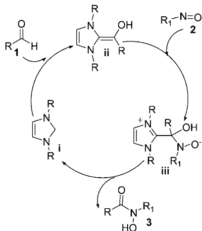
Scheme 1. Proposed Amidation of Aldehydes Using Nitrosobenzene
