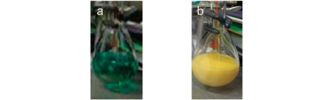
Figure 1. NHC-catalyzed synthesis of N -hydroxy-4-nitro- N -phenyl benzamide ( 3c ). Scale up of 5 g product (a) before activation of the catalyst ( 4 , 0.125 mol %), and (b) after reaction completion (in 2 min).
