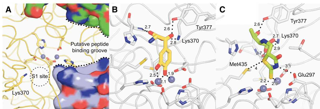
Fig. 6. Modeling of selected inhibitors in the DNPEP active site. (A) Structure of the DNPEP active site (PDB accession code 3VAT) showing the binuclear zinc center (gray spheres) in relation to the S1 site and the peptide-binding groove of the enzyme, which is partially formed by additional subunits of the DNPEP complex (shown in surface representation). Lys 370 , present in the S1 site of the enzyme, confers selectivity by interacting with the negatively charged N-terminal Asp or Glu residue of DNPEP peptide substrates. Models of (B) compound 241320 and (C) compound 347749 binding to the DNPEP active site. The model in (B) was docked based on the structure of methionine aminopeptidase in complex with a catechol-containing inhibitor (Wang et al., 2008), whereas the model in (C) was placed assuming that the exocyclic double-bonded sulfur atom is the relevant metal chelator in this compound. Both models were energy minimized using the Crystallography and NMR System program (Brunger, 2007). Distances are given in angstroms.
