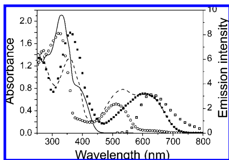
Figure 4. Absorption spectra of a 2-methyltetrahydrofuran solution of triad 1 after irradiation with light to produce solutions very highly enriched in FGo-DTEo (—), FGc-DTEo (○), FGo-DTEc (■), and FGc-DTEc (---). Also shown is the fluorescence emission at 630 nm from the fulgimide in FGc-DTEo excited at 500 nm (□).
