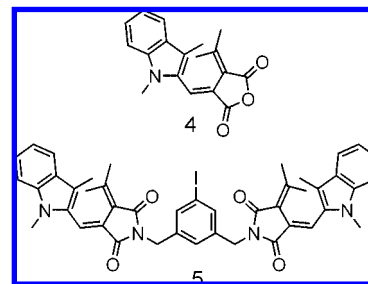
Figure 9. Structures of synthetic intermediate fulgide 4 and fulgimide 5 .
