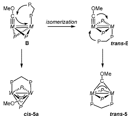
Scheme 2. Pathways in the Reactions of Compounds 1a,b with dmpm ( \text{M} = \text{WCp}, \text{MoCp} ; \text{P} = \text{PPh}_2, \text{PEt}_2 ; \text{P--P} = \text{Me}_2\text{PCH}_2\text{PMe}_2 or dmpm; positive charges in all complexes omitted for clarity)
