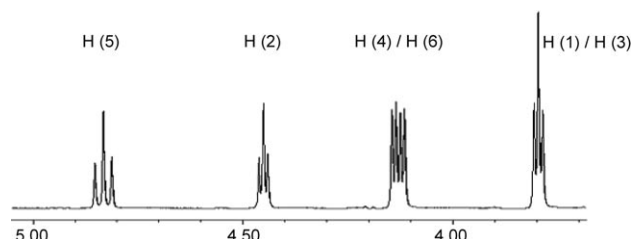
Figure 4. The cyclohexane region of the 600 MHz ^1H NMR spectrum of 2 .
