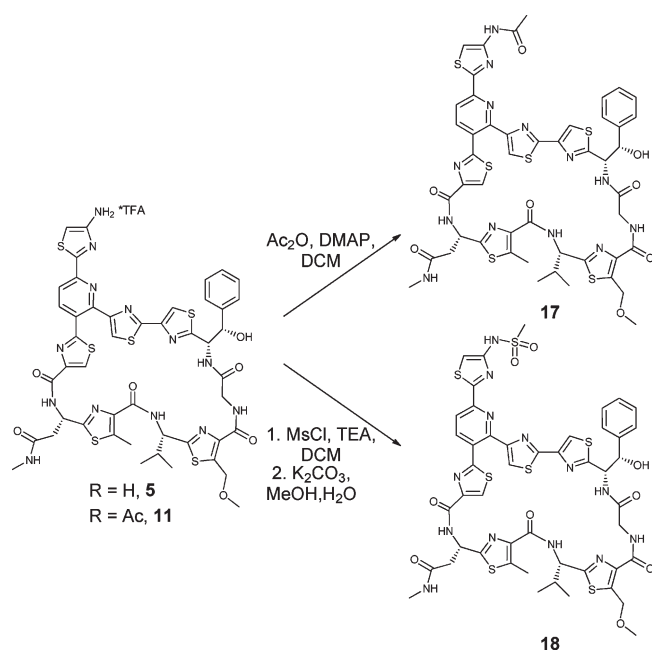
Scheme 4. 4-Aminothiazole Stabilization
