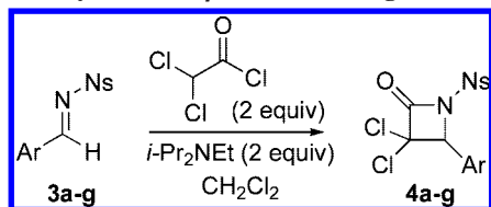
SCHEME 2. Synthesis of \beta -Lactams 4a–g
