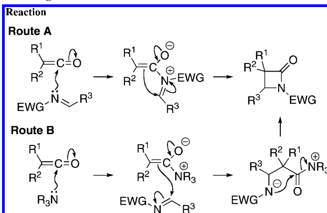
SCHEME 8. Mechanistic Routes Using Dichloroketene
