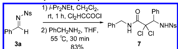
SCHEME 5. Synthesis of \beta -Aminoamide 7
