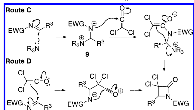
SCHEME 8. Mechanistic Routes Using Dichloroketene
