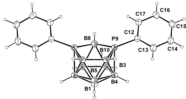
Fig. 1. ORTEP drawing of the structure of 7,9-Ph 2 -nido-7,9-P 2 B 9 H 9 ( 1 ). Selected bond distances (Å): P9–B8, 1.917(2); P9–B10, 1.923(3); P9–C12, 1.796(2); P9–B4, 2.028(3); P9–B3, 2.061(3); B1–B3, 1.758(4); B1–B4, 1.770(3); B1–B5, 1.785(5); B3–B3', 1.748(5); B3–B4, 1.843(4); B3–B8, 1.875(4); B4–B5, 1.753(3); B4–B10, 1.860(4); B5–B10, 1.778(4); B10–B10', 1.740(5).
