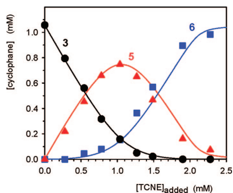
Figure 3. Cyclophane distribution at varying added [\text{TCNE}] and at fixed 1.03 \text{ mM} overall cyclophane concentration. Points are experimental, and curves are calculated.
