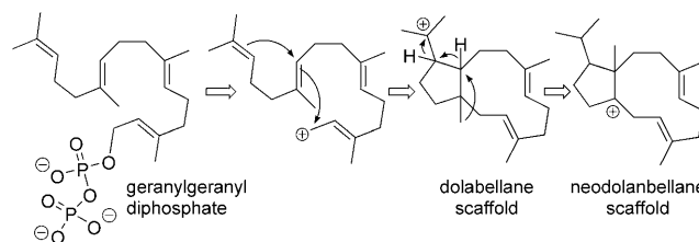
Figure 1. Proposed biosynthesis of dolabellanes and neodolabellanes.
