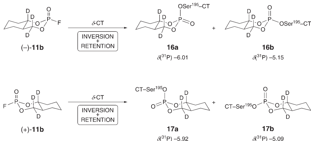
Scheme 10
