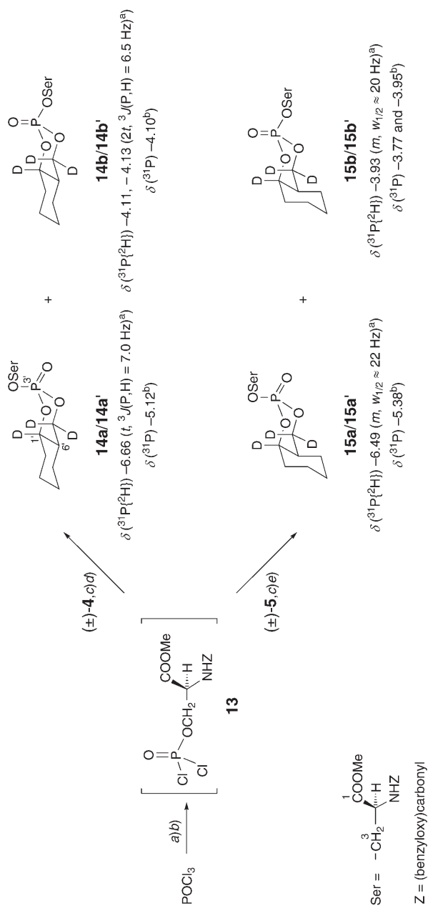
Scheme 5
