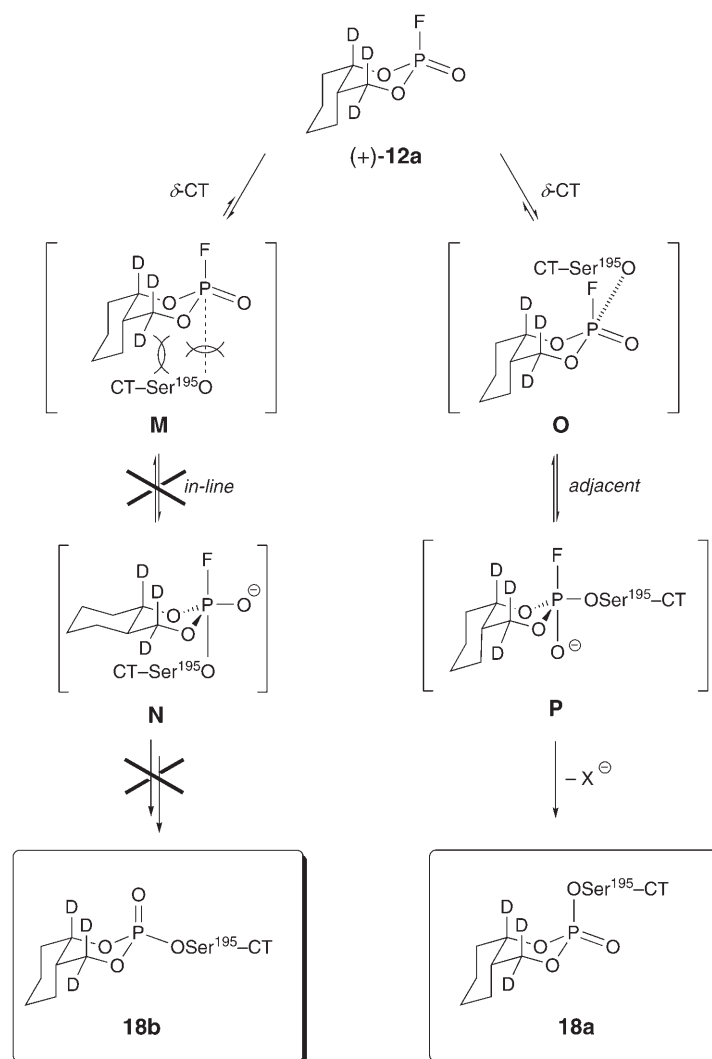
Scheme 14
