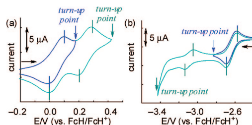
Figure 3. Cyclic voltammograms of disilene 1 (V vs FcH/FcH + ): (a) oxidation region measured in 0.1 M Bu 4 NB(C 6 F 5 ) 4 in o -dichlorobenzene ( E 1/2 (FcH/FcH + ) = +0.34 V vs Ag/Ag + ); (b) reduction region measured in 0.1 M Bu 4 NBF 4 in THF ( E 1/2 (FcH/FcH + ) = +0.57 V vs Ag/Ag + ). The scan rate was 0.01 V/s.
