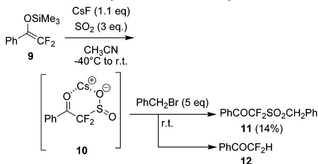
SCHEME 5. Decomposition of Sulfinate 10
