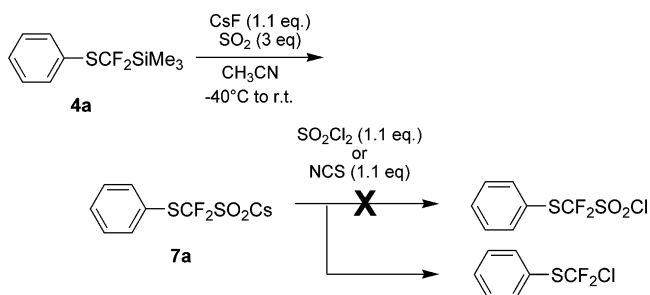
SCHEME 6. Chlorination of 7a
