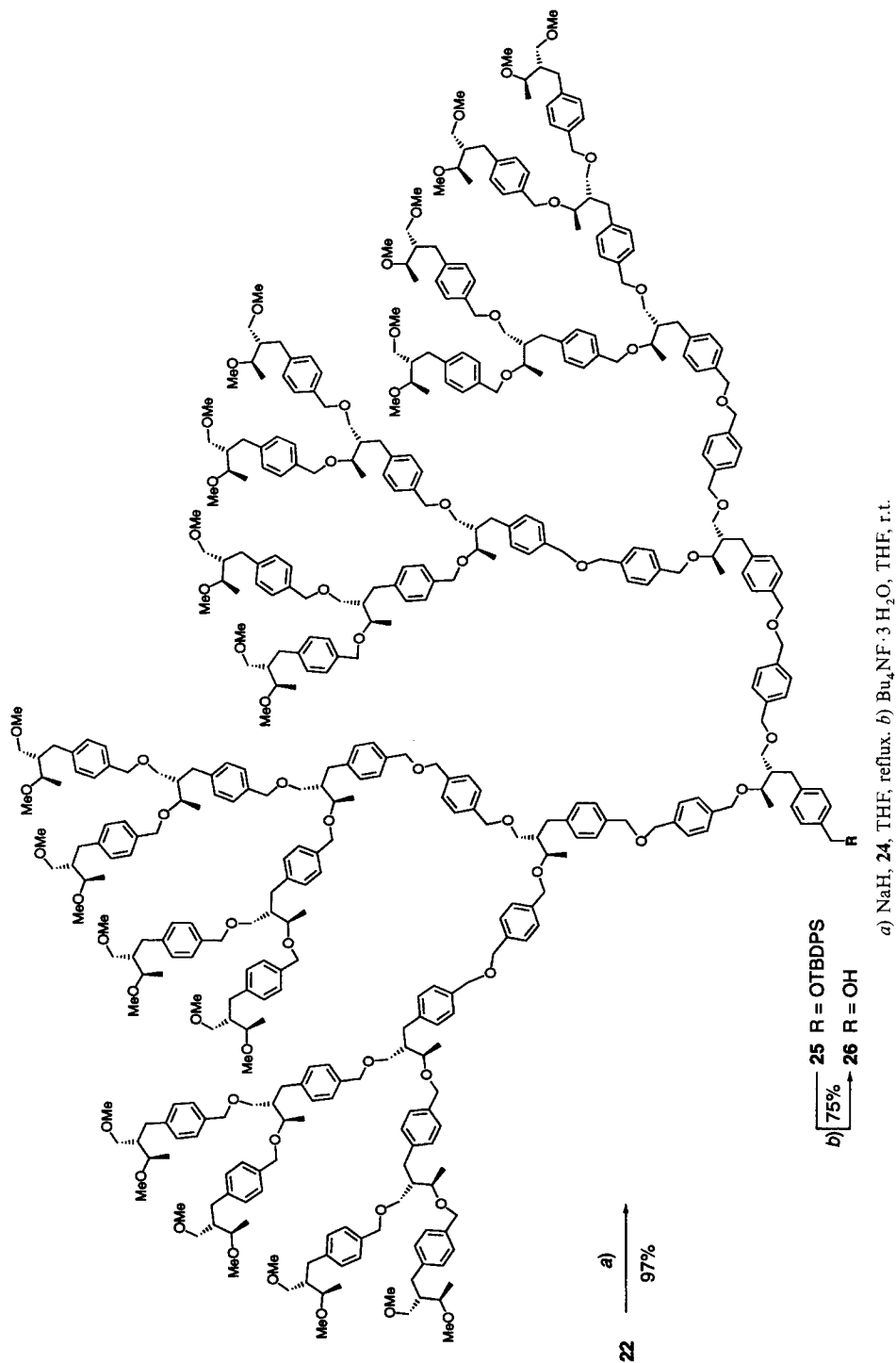
Scheme 4. Preparation of the 5th-Generation Benzyl-Alcohol Branch 26
