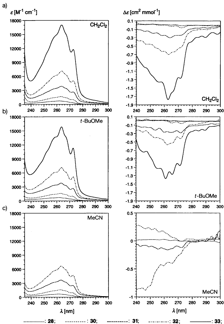
Fig. 11. UV (left) and CD spectra (right) of dendrimers 28 , 30 , 31 , 32 , and 33 of 0th to 4th generation in a) \text{CH}_2\text{Cl}_2 , b) t\text{-BuOMe} , and c) \text{MeCN} . c = 10^{-3} - 10^{-4} \text{ M} at room temperature.
