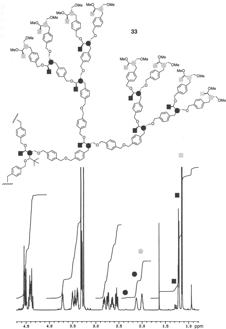
Fig. 4. Part of the 500-MHz ^1\text{H} -NMR spectrum of the 4th-generation dendrimer 33 measured in \text{CDCl}_3 . The labelling of signals or groups of signals refers to the sets of Me groups (depicted as rectangles) and of CH groups (depicted as circles) in the corresponding formula.
