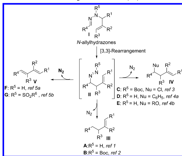
Scheme 1. [3,3]-Rearrangement of N -Allylhydrazones
