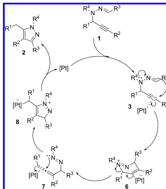
Scheme 4. Proposed Mechanism
