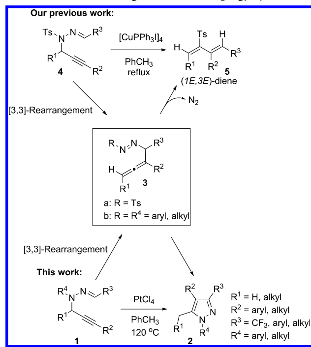
Scheme 2. [3,3]-Rearrangement of N -Propargylhydrazones
