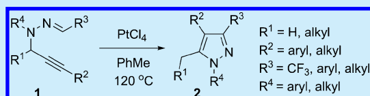
Scheme 2. [3,3]-Rearrangement of N -Propargylhydrazones
