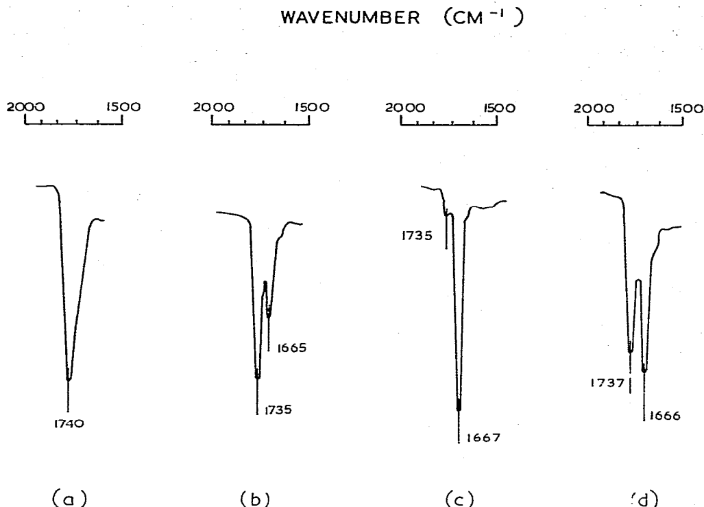
Fig. 3. The carbonyl region infrared spectra of monobutyltin isooctylthioglycolates and monobutyltin isooctylthioglycolate chlorides: (a) \text{BuSn(IOTG)}_3 ; (b) Initial mixture from the reaction between butyltin trichloride and 3 moles of isooctylthioglycolate at 95^\circ\text{C} ; (c) \text{BuSnCl}_2(\text{IOTG}) ; (d) \text{BuSnCl(IOTG)}_2 .
