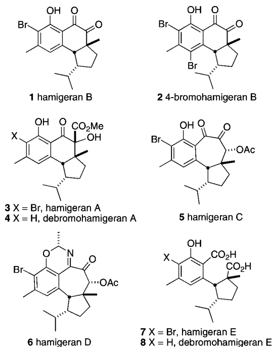
FIGURE 1. Structures of hamigerans.
