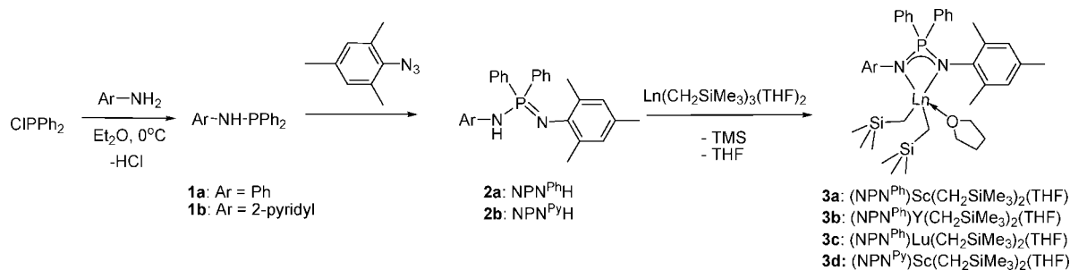
Scheme 1. Synthesis of Complexes 3a–d
