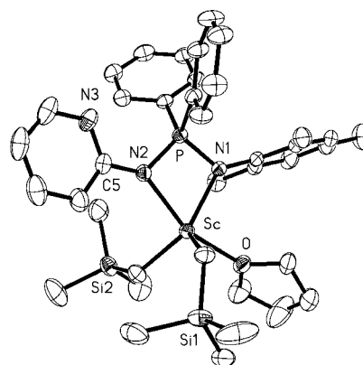
Figure 4. X-ray structure of 3d with 35% probability thermal ellipsoids. Hydrogen atoms are omitted for clarity. Selected bond lengths (Å) and angles (deg): Sc–N(1) = 2.1780(17), Sc–N(2) = 2.2021(18), Sc–O = 2.1974(16), Sc–C(32) = 2.222(2), Sc–C(36) = 2.232(2), Sc–P = 2.8942(7), N(1)–P = 1.6164(18), N(2)–P = 1.6246(18), N(3)–C(5) = 1.342(3), N(2)–C(5) = 1.397(3), N(1)–Sc–N(2) = 67.37(6), C(31)–Sc–C(35) = 111.88(9), O–Sc–C(31) = 95.05(8), O–Sc–C(35) = 94.11(8), Sc–C(31)–Si(1) = 124.79(12), Sc–C(35)–Si(2) = 131.76(13).
