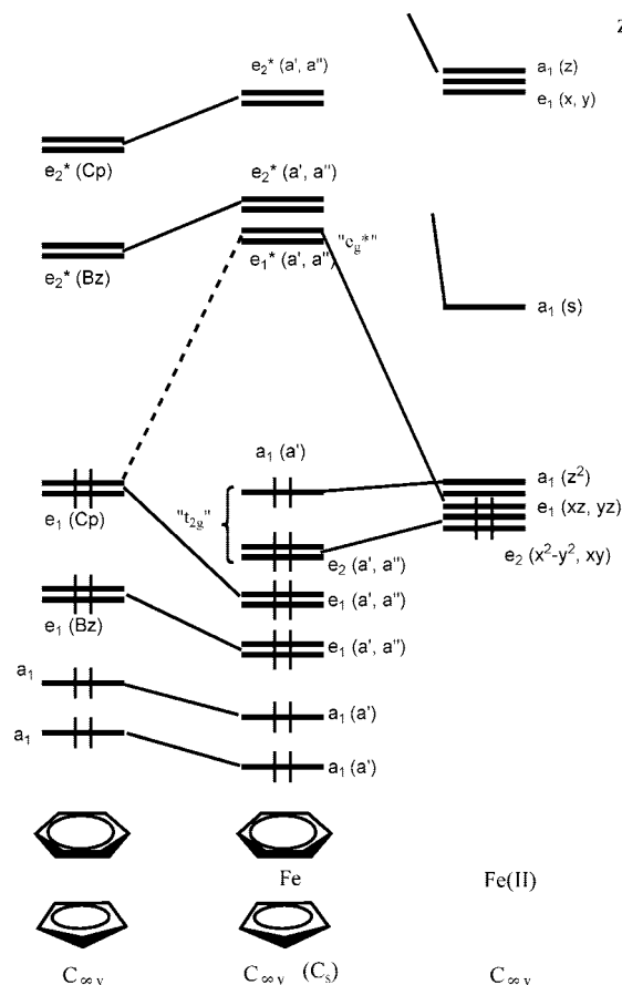
Figure 5. Qualitative MO interaction diagram for \text{CpFe}(\text{C}_6\text{H}_6)^+ ( \text{C}_{\infty v} : pseudosymmetry; \text{C}_s : exact symmetry).
