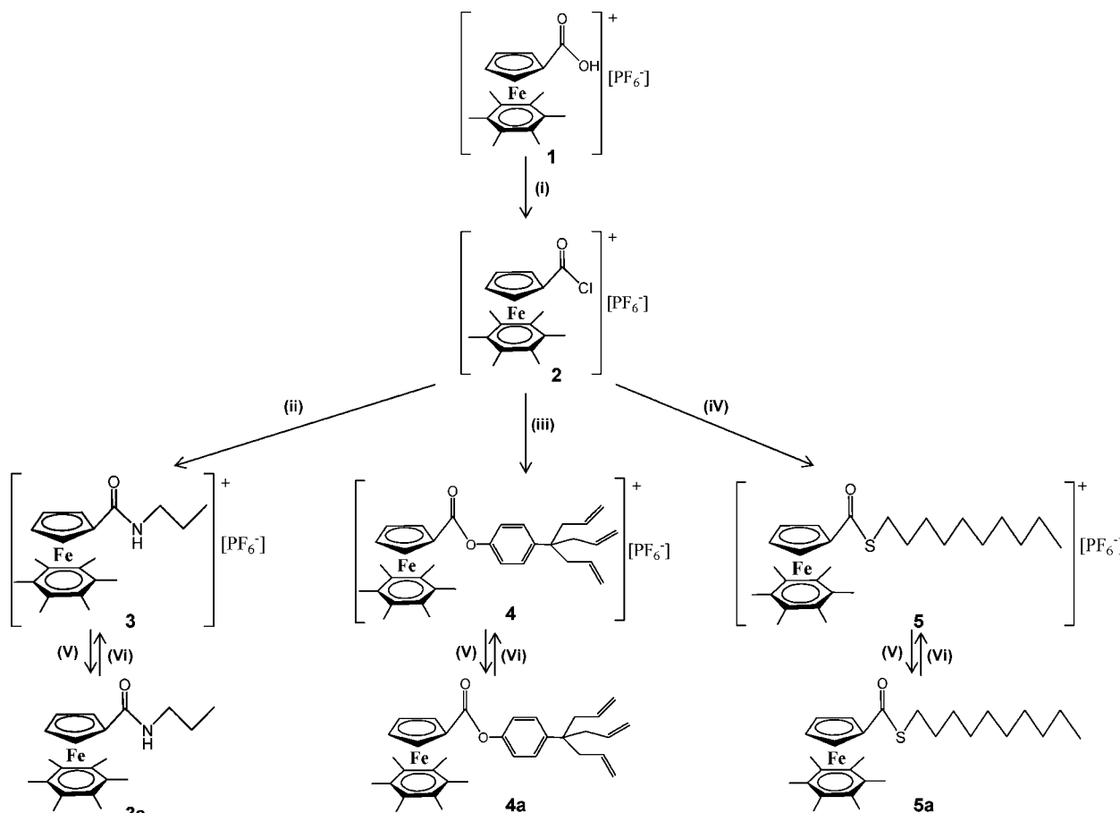
Scheme 1. Synthesis of [(\eta^5\text{-C}_5\text{H}_4\text{COR})\text{Fe}^{\text{II}}(\eta^6\text{-C}_6\text{Me}_6)][\text{PF}_6] and Their Reduction to 19-Electron Forms a
