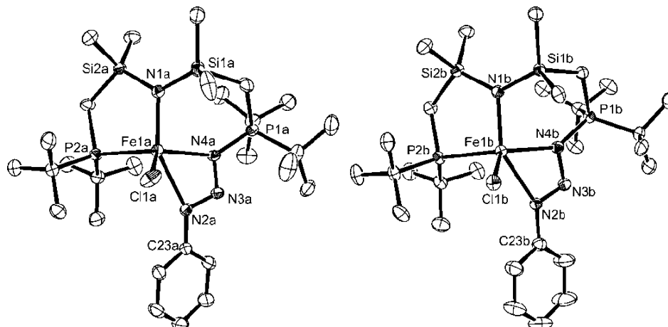
Figure 2. ORTEP drawing (50% probability) of the non-hydrogen atoms of [\text{tBu}_2\text{PCH}_2\text{SiMe}_2\text{NSiMe}_2\text{CH}_2\text{P}'\text{Bu}_2\text{N}_3\text{Ph}]\text{FeCl} , showing selected atom labeling of molecules a and b. Unlabeled atoms are carbon. Selected structural parameters (molecules a and b): Fe1–N1, 2.0439(17) and 2.0359(16) Å; Fe1–N2, 2.4422(17) and 2.3283(16) Å; Fe1–N4, 2.1290(17) and 2.2099(16) Å; Fe1–Cl 1, 2.2971(6) and 2.3062(6) Å; Fe1–P2, 2.4860(6) and 2.5015(6) Å; P1–N4, 1.6538(17) and 1.6587(16) Å; N2–N3, 1.271(2) and 1.278(2) Å; N2–C23, 1.422(3) and 1.421(3) Å; N3–N4, 1.360(2) and 1.347(2) Å.
