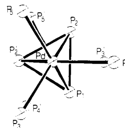
Figure 4. View of the coordination polyhedron of [(\text{triphos})\text{Pd}(\mu\text{-(}\eta^3\text{-P}_3\text{))Pd}(\text{triphos})]^+ along the pseudoternary axis.
