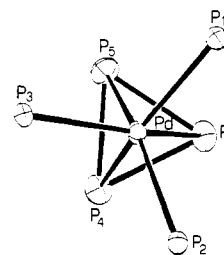
Figure 2. View of the coordination polyhedron of [(\text{triphos})\text{Pd}(\eta^3\text{-P}_3)]^+ along the pseudoternary axis.
