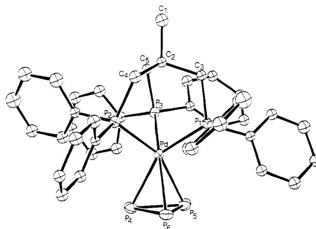
Figure 1. Perspective view of the [(\text{triphos})\text{Pd}(\eta^3\text{-P}_3)]^+ cation.
