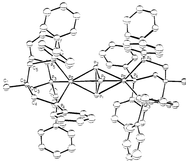
Figure 3. Perspective view of the [(\text{triphos})\text{Pd}(\mu\text{-(}\eta^3\text{-P}_3\text{))Pd}(\text{triphos})]^+ cation.
