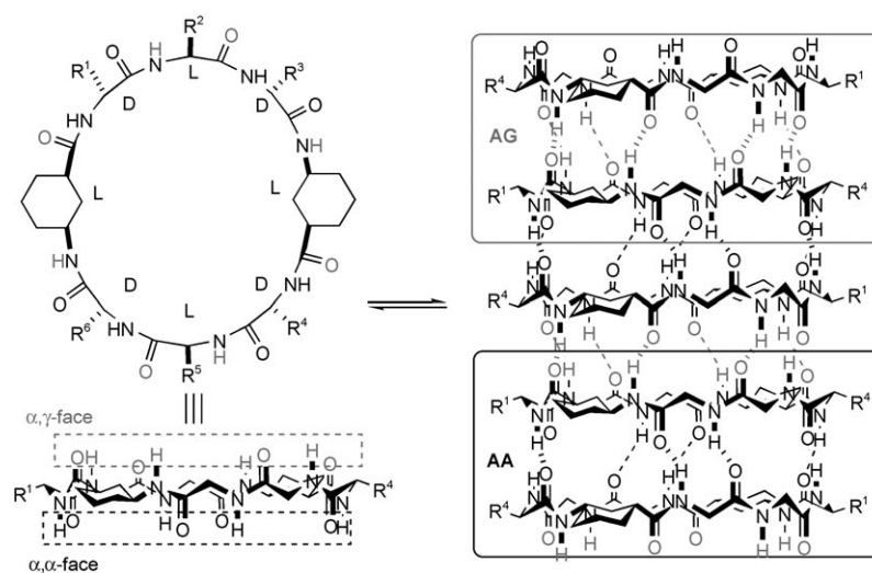
Figure 3. AA- and AG-type hydrogen bonding between cyclo-[(L- \gamma -Ach-D-Aa-L-Aa-D-Aa) 2 ]- units (for clarity, most amino acid side chains have been omitted in the representation of the nanotube).
