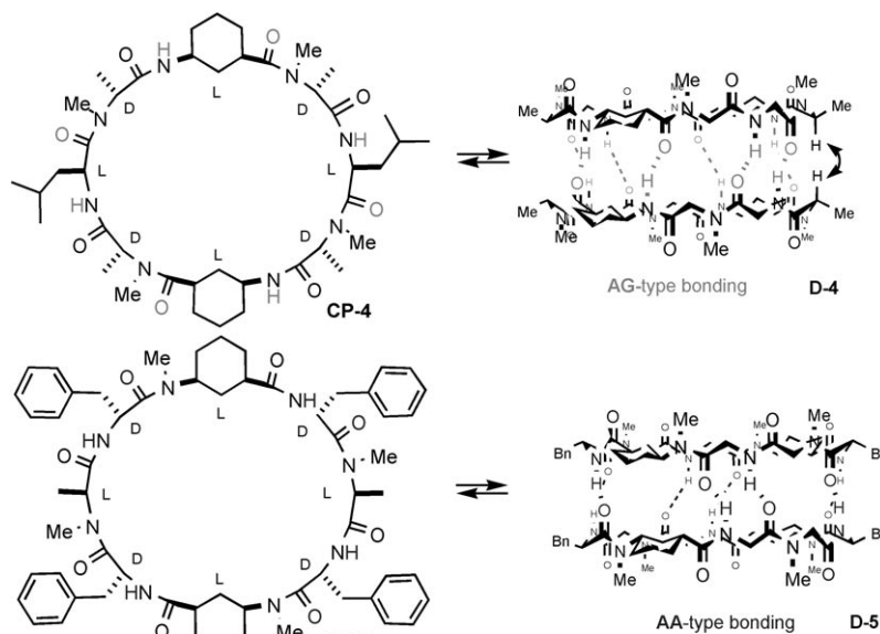
Figure 4. Cyclic peptides CP-4 and CP-5 and their corresponding dimers (for clarity, most amino acid side chains have been omitted from the representations of the dimers).
