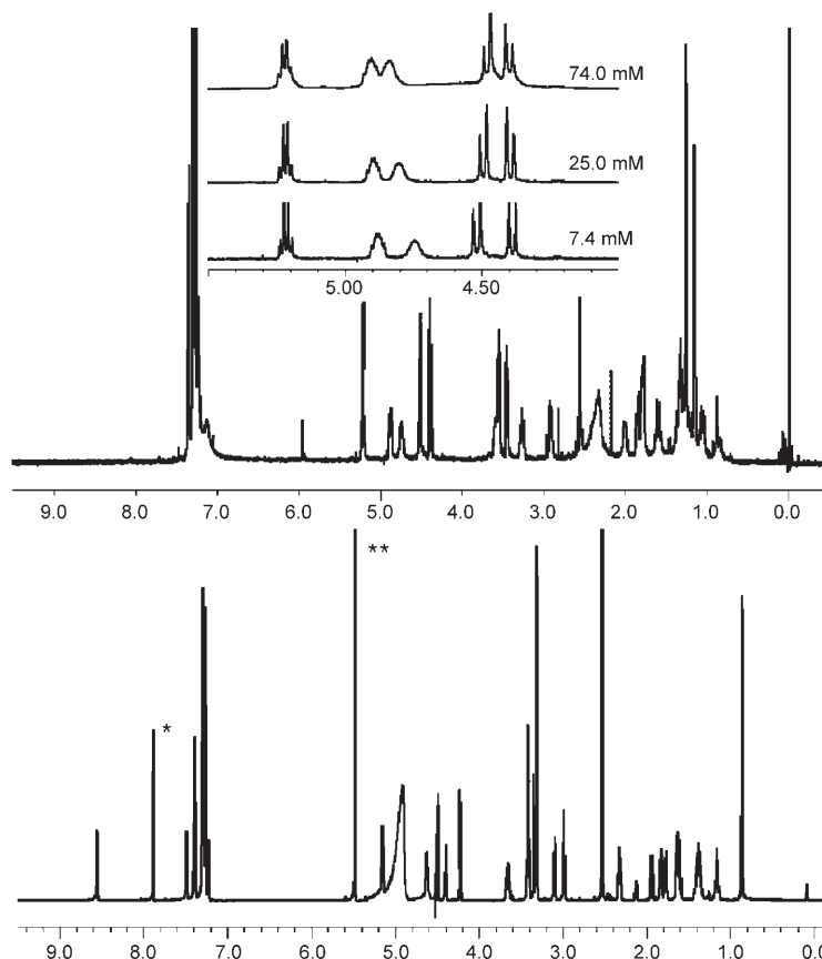
Figure 10. Top: 1 H NMR spectrum of a solution of peptide CP-10 in CDCl 3 (7.4 mM) with the 4.0–5.5 ppm region of the spectra of 74.0, 25.0 and 7.4 mM solutions, showing the downfield shift of Phe H \alpha . Bottom: 1 H NMR spectrum of a solution of peptide CP-10 in CD 3 OH (10 mM). [* CHCl 3 (7.89 ppm), ** CH 2 Cl 2 (5.48 ppm)].
