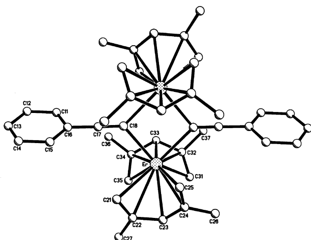
Fig. 2. The structure of [(2,4\text{-C}_7\text{H}_{11})_2\text{ErC}\equiv\text{CC}_6\text{H}_5]_2 .
