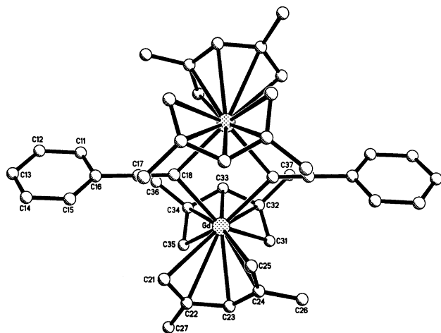
Fig. 1. The structure of [(2,4\text{-C}_7\text{H}_{11})_2\text{GdC}\equiv\text{CC}_6\text{H}_5]_2 .
