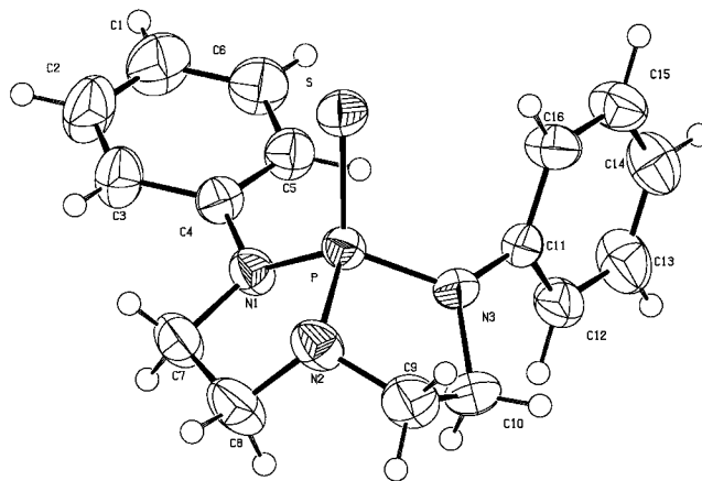
FIGURE 1 ORTEP drawing of 2a .
