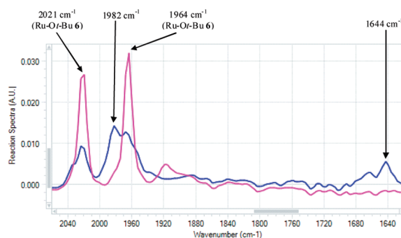
Figure 5. FT-IR spectra before (pink, t = 0 min) and after (blue, t = 29 min) the addition of 5-hexene-2-ol ( 4 ) to tert -butoxide complex 6 .
