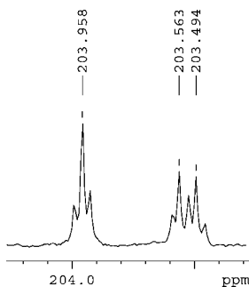
Figure 3. Carbonyl signals of ^{13}\text{CO} -labeled complexes a and b (55% ^{13}\text{CO} ).
