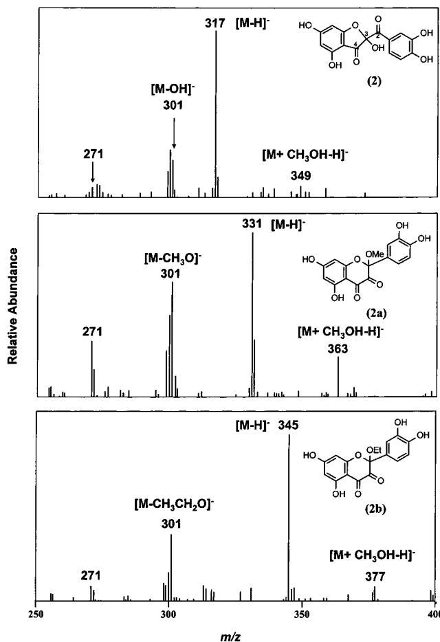
Figure 3. Atmospheric pressure chemical ionization mass spectra of the substituted 3(2H)benzofuranone ( 2 ), and the methoxylated ( 2a ) and ethoxylated adducts ( 2b ).
