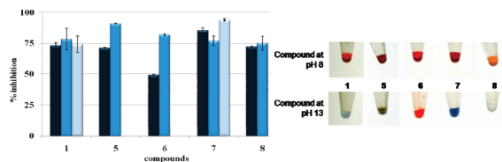
Figure 2. Left panel: Screening of 1 , 5–8 ( 5\ \mu\text{M} ) against pure mNat2 (dark blue columns), hNat1 in Escherichia coli cell lysate (blue columns), and hNat1 in breast cancer cell lysate (ZR-75-1 cells, 1 and 7 only, light blue columns). NAT activity was determined as acetylation of p Aba in the presence of AcCoA. Right panel: Compounds 1 , 5–8 ( 2\ \text{mM} ) in Tris-HCl buffer (pH 8.0, top) or aq. NaOH (bottom).
