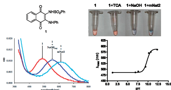
Figure 1. Top right: 1 (400 \mu M) in aq. Tris·HCl (pH 8.0); 20% trichloroacetic acid (TCA); 4 M aq. NaOH; or mNat2 in aq. Tris·HCl (pH 8.0). Bottom left: Visible spectra of 1 (10 \mu M) in aq. Tris·HCl (pH 8.0, red line, \lambda_{\text{max}} = 489 nm), 1 in aq. NaOH solution (dark blue line, \lambda_{\text{max}} = 561 nm), and 1 with 2 equiv of mNat2 in aq. Tris·HCl (pH 8.0, light blue line, \lambda_{\text{max}} = 610 nm). Bottom right: pH titration curve for 1 ( pK_a ~9.5).
