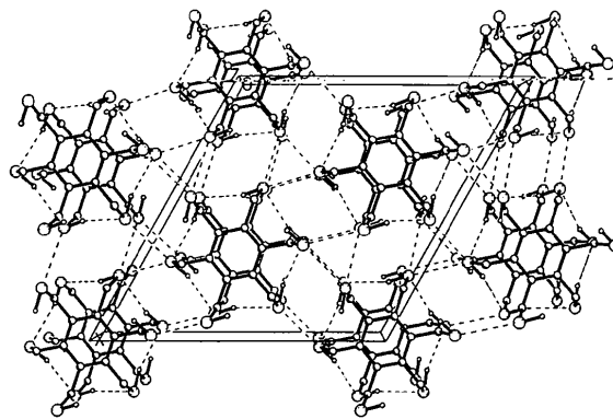
Fig. 2. A view along c showing the packing of (1) in its molecular crystal. S—H \cdots S hydrogen bonds and S \cdots S intermolecular interactions are indicated by dotted/dashed and dashed lines, respectively.
