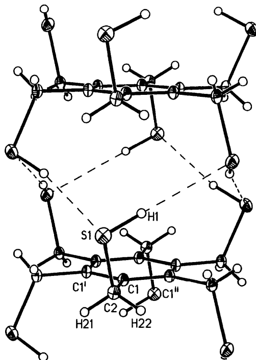
Fig. 1. A view normal to the c axis showing the juxtaposition of molecules of (1) along c . Displacement ellipsoids are drawn at the 50% probability level. The S—H \cdots S hydrogen bonds are represented by dashed lines.
