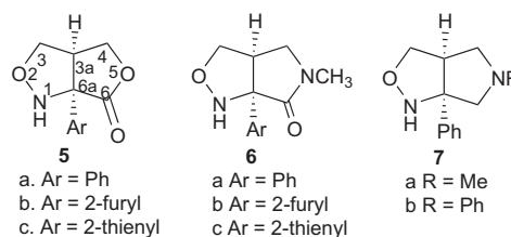
Fig. 2. Isioxazolo-fused bicyclic organocatalysts.
