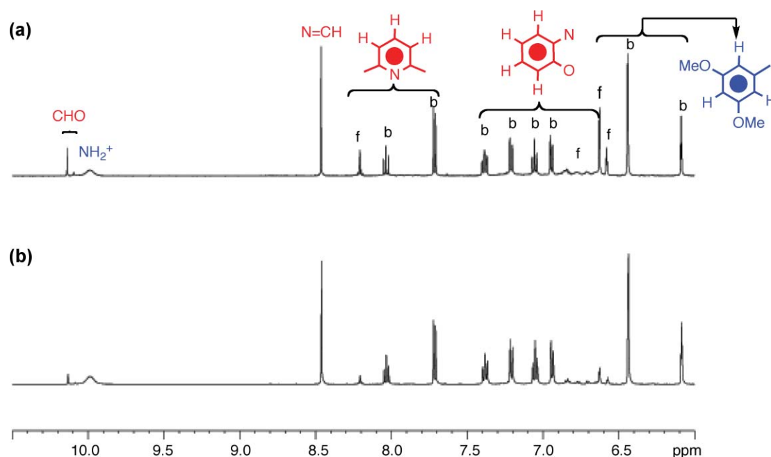
Fig. 3 Partial ^1\text{H} NMR spectra (500 MHz, \text{CD}_3\text{CN} , 298 K, aromatic region) of the dissociated dynamic [2]rotaxane 1a -H- \text{PF}_6 (b = bound and f = free) after treatment with (a) anhydrous \text{MgSO}_4 and (b) anhydrous \text{Na}_2\text{SO}_4 , evaporated and redissolved in MeCN through three consecutive cycles.
