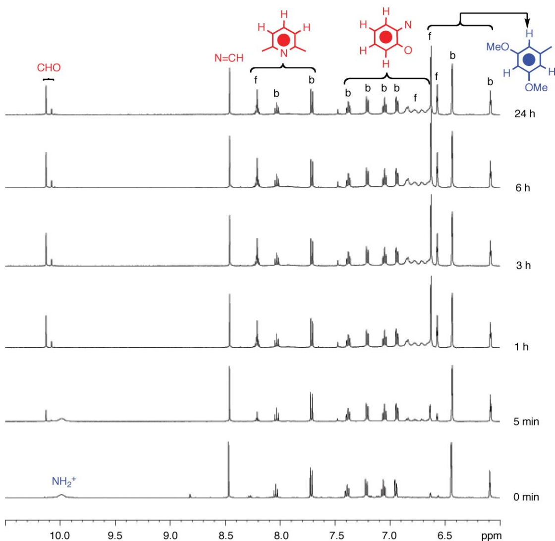
Fig. 1 Partial ^1\text{H} NMR spectra (aromatic region, 500 MHz, \text{CD}_3\text{CN} , 298 K, 200 mol equivalents of \text{D}_2\text{O} , total conc. = 16.6 mM) showing the dissociation of the dynamic [2]rotaxane 1a - \text{H}\cdot\text{PF}_6 with time (b = bound rotaxane and f = free components). With increasing time, the characteristic proton signals originating from the aldehyde ( \delta = 10.12 ppm), the free (f) pyridine ring ( \delta = 8.22 ppm) and the free (f) dimethoxyaryl ring ( \delta = 6.62 and 6.58 ppm) in separate cyclic (or acyclic) and dumbbell components were found to have their relative intensities increase while those signals arising from the rotaxane decreased. The results indicate that the dynamic [2]rotaxane dissociates slowly into its free components— 2 , 3a and 4 - \text{H}\cdot\text{PF}_6 —until the dissociation process has reached equilibrium after 24 h. With particular reference to 1a - \text{H}\cdot\text{PF}_6 , there was 41% of the dynamic [2]rotaxane remaining in the mixture after 24 h.
