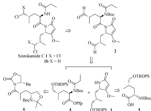
Figure 1. Retrosynthetic analysis.
