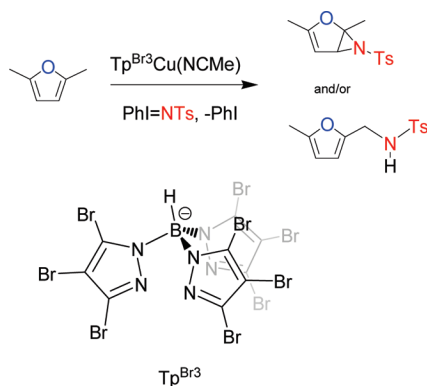
Scheme 2. Expected Products Derived from the Reaction of 2,5-Dimethylfuran and \text{PhI}=\text{NTs}
