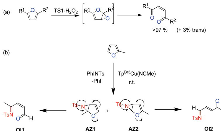
Scheme 6. Transimination Pathway That Converts OI1 into OI2
