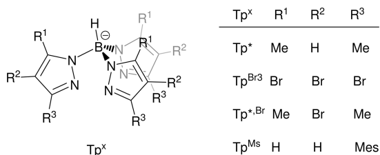
Scheme 3. Ligands Employed in This Work
