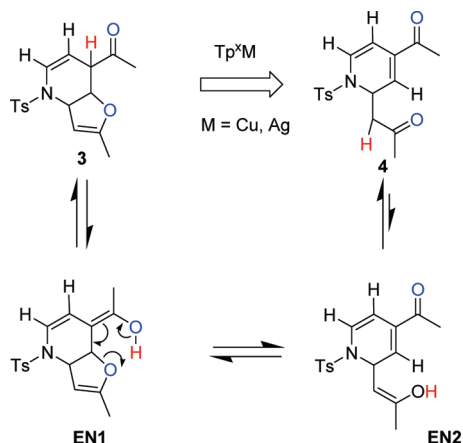
Scheme 9. Overall Mechanism for the Concurrent Tandem Catalytic System to Convert 2-Methylfuran and PhI=NTs into Dihydropyridine 4
