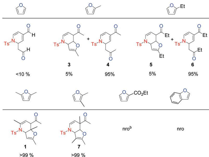
Scheme 4. Reactivity of Several Furans with \text{PhI}=\text{NTs} in the Presence of \text{Tp}^{\text{Br}^3}\text{Cu}(\text{NCMe}) as the Catalyst a,b
