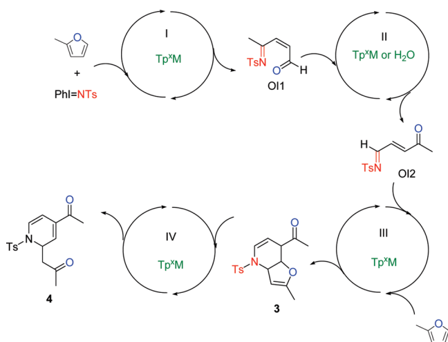
Scheme 9. Overall Mechanism for the Concurrent Tandem Catalytic System to Convert 2-Methylfuran and PhI=NTs into Dihydropyridine 4
