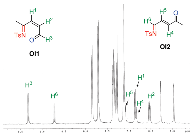
Figure 2. ^1\text{H} NMR spectrum ( \text{CDCl}_3 , 400 MHz) of the reaction of 2-methylfuran and \text{PhI}=\text{NTs} (equimolar ratio) using \text{Tp}^{\text{Br}^3}\text{Cu}(\text{NCMe}) as the catalyst after 10 min of stirring at room temperature.
