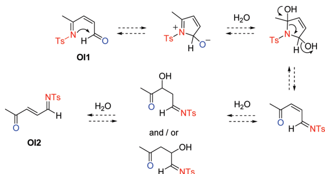
Scheme 6. Transimination Pathway That Converts OI1 into OI2
