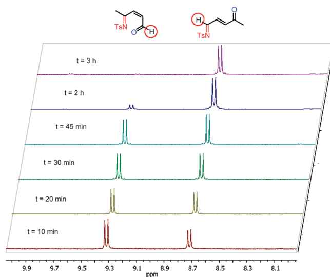
Figure 3. Monitoring of the reaction mixture of 2-methylfuran and \text{PhI}=\text{NTs} (equimolar ratio) using \text{Tp}^{\text{Br}^3}\text{Cu}(\text{NCMe}) as the catalyst with time (downfield region).
