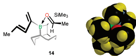
Figure 1. Pretransition state complex 14 with Spartan 06-generated space-filling model.
