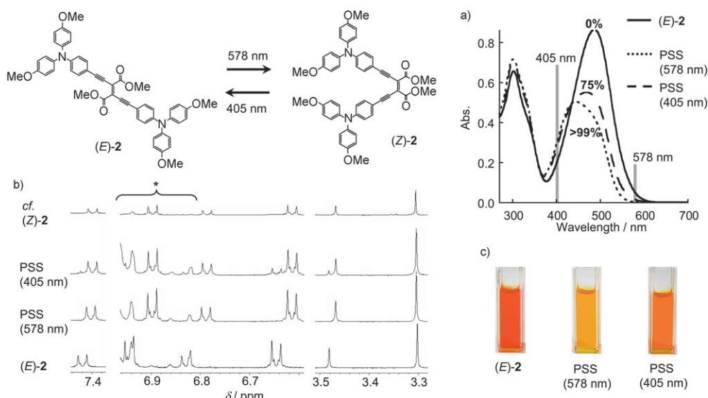
Figure 6. a) UV/Vis and b) ^1\text{H} NMR spectral changes of ( E )- 2 in toluene and [\text{D}_8]\text{toluene} , respectively, upon irradiation with light at 578 and 405 nm. The percentages given in a) indicate the proportion of the Z isomer in each state. The asterisk in b) indicates the presence of signals derived from the solvent. The scale for the methoxy protons is reduced to one-third of that for the aromatic protons. c) Photograph of ( E )- 2 before and after irradiation with light at 578 or 405 nm.
