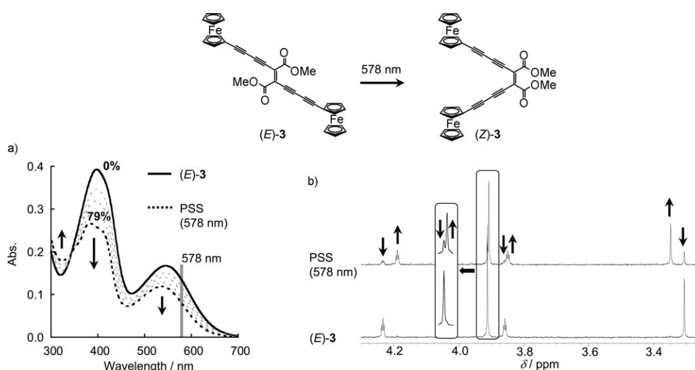
Figure 7. a) UV/Vis and b) 1 H NMR spectral changes of ( E )- 3 in toluene and [D 8 ]toluene, respectively, upon irradiation with light at 578 nm. The percentages given in a) indicate the proportion of the Z isomer in each state.
