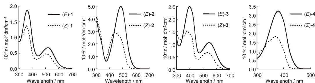
Figure 4. Overlays of the electronic spectra of the E and Z forms of 1–4 in toluene. Those of the Z forms were measured directly for 1 , and calculated mathematically from photoirradiation experiments described in a later section.
