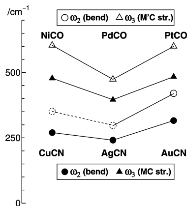
Figure 4. Comparison of the vibrational frequencies in the group 11 monocyanides MCN (M = Cu, 18 Ag, and Au) and the isoelectronic group 10 monocarbonyls M'CO (M' = Ni, 35 Pd, 36 and Pt 37,38 ). The \omega_2 values for NiCO and PdCO refer to theoretical calculations. 39,40
